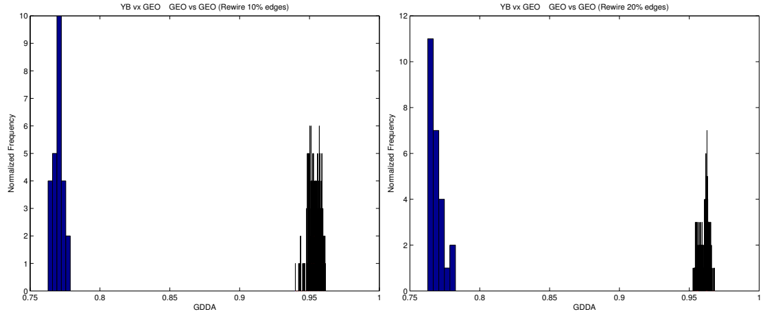
(a) YB vs. GEO-3D and GEO-3D vs. GEO-3D (rewired 10% edges) (b) YB vs. GEO-3D and GEO-3D vs. GEO-3D (rewired 20% edges)
